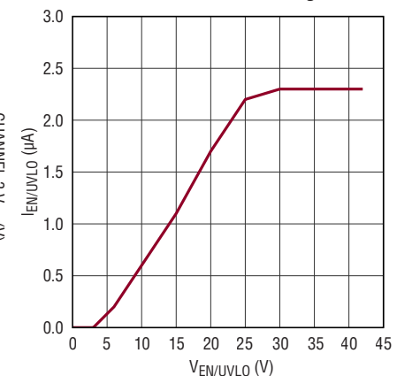
EN/UVLO Current vs Voltage
