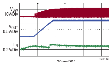
Single Phase Start-Up with No load
