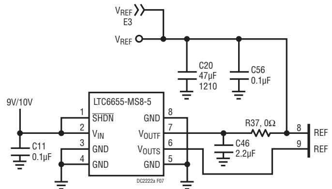
Figure 7. Reference Circuit
