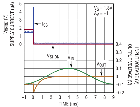
Shutdown Transient with Sinusoidal Input
