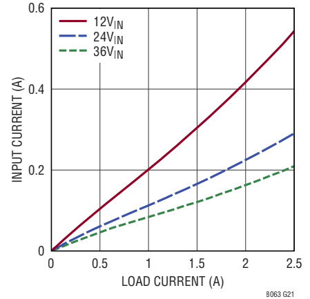
Input vs Load Current V_{OUT} = 2\text{V}
