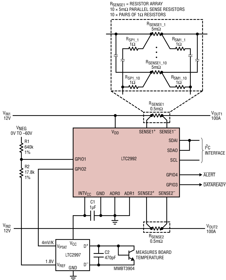
Dual 12V High Power Monitor with One Negative Voltage Monitor
