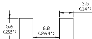
REFLOW SOLDER
