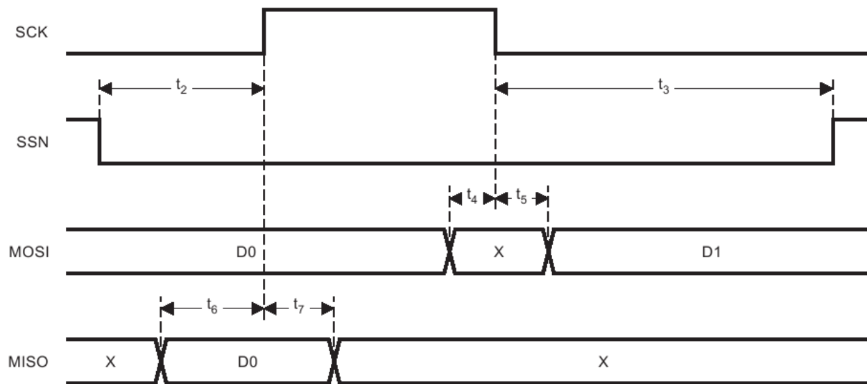
Figure 4 Slave Timing
