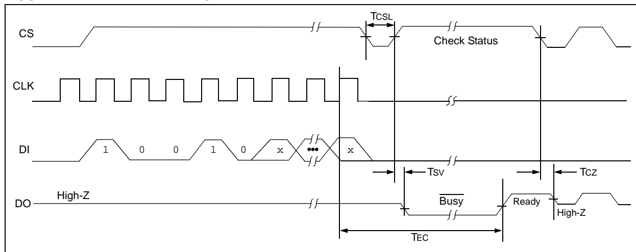
FIGURE 2-2: ERAL TIMING
