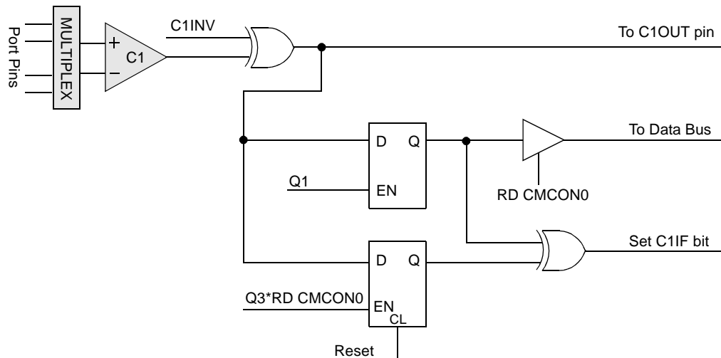
FIGURE 7-3: COMPARATOR C1 OUTPUT BLOCK DIAGRAM (PIC16F636/639)
