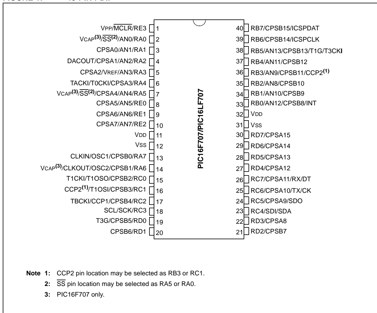
FIGURE 1: 40-PIN PDIP
