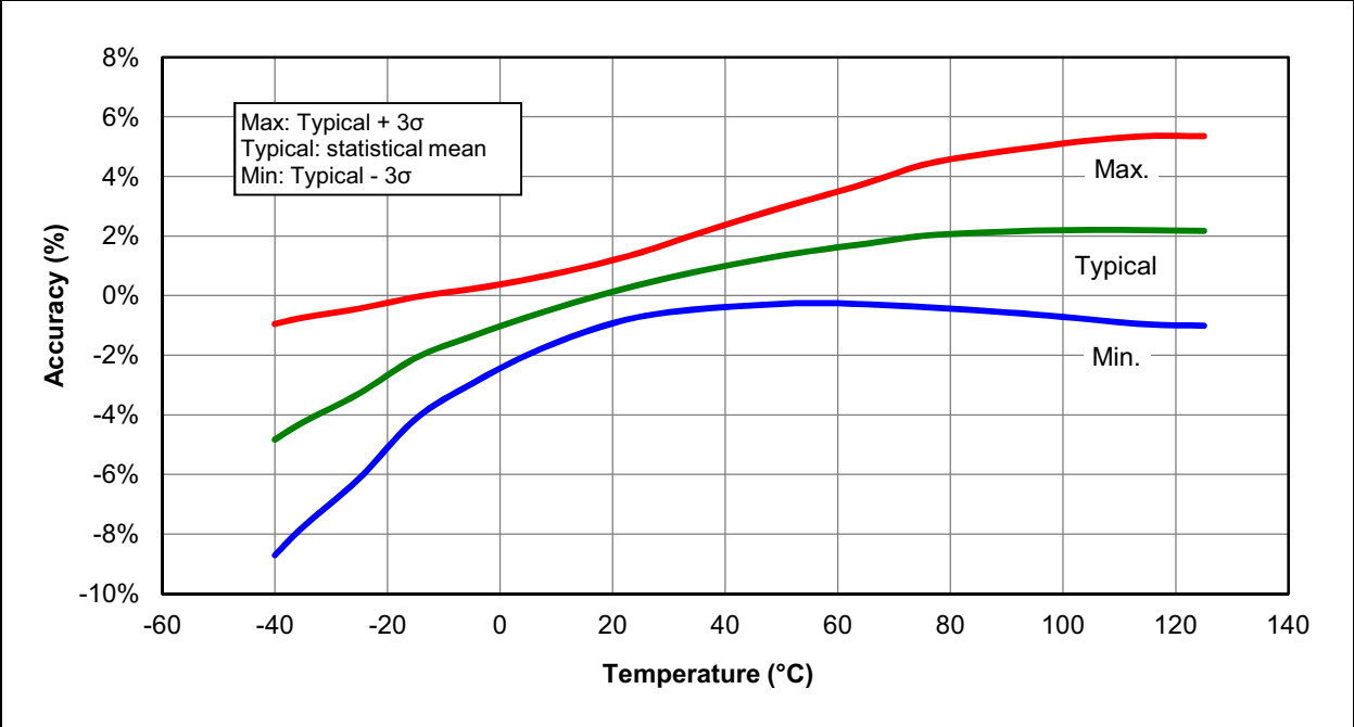
FIGURE 28-61: HFINTOSC ACCURACY OVER TEMPERATURE, 2.3V ≤ VDD ≤ 5.5V
