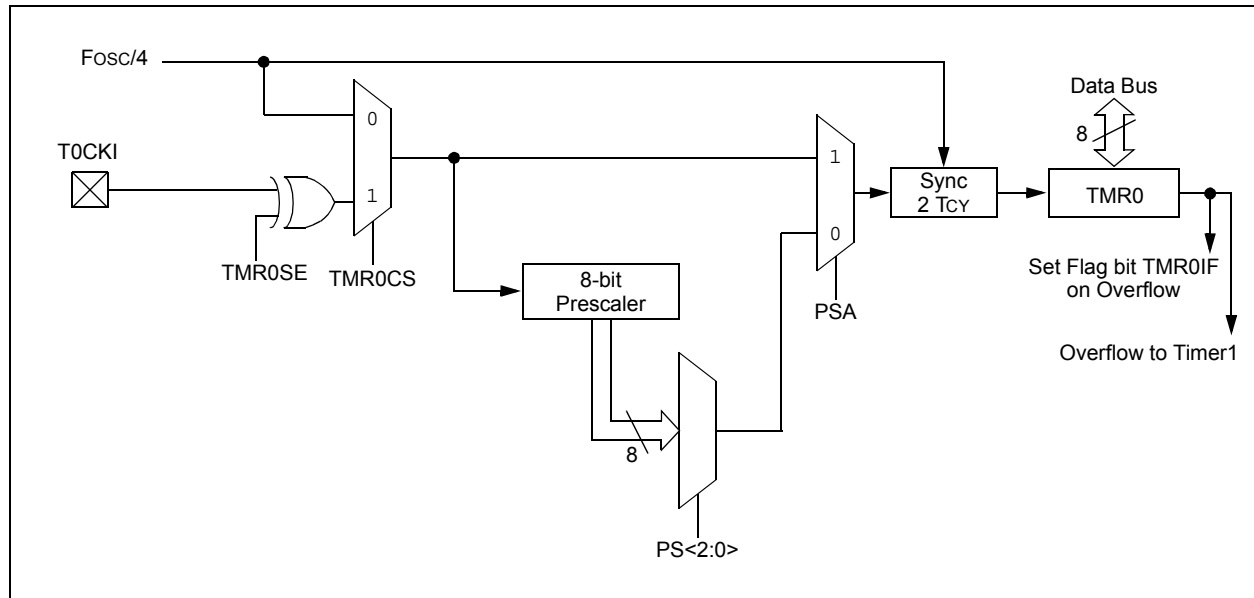
FIGURE 17-1: BLOCK DIAGRAM OF THE TIMER0
