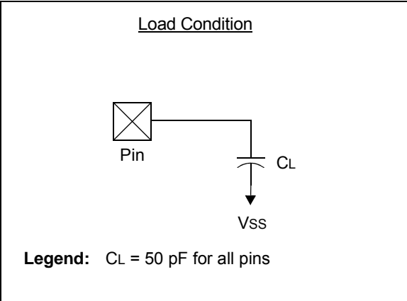
FIGURE 21-3: LOAD CONDITIONS
