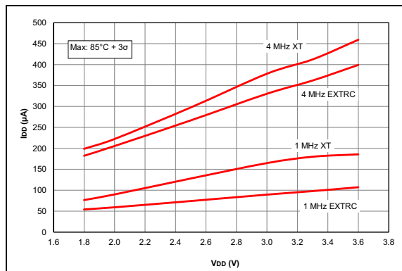
FIGURE 32-4: I_{DD} Maximum, XT and EXTRC Oscillator, PIC16F1788/9 Only.
