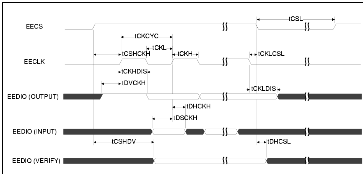
FIGURE 6-10: EEPROM TIMING
