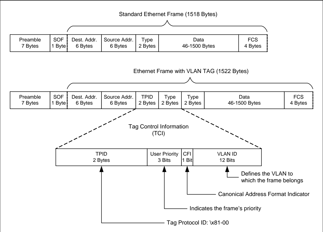
FIGURE 9-1: VLAN FRAME
