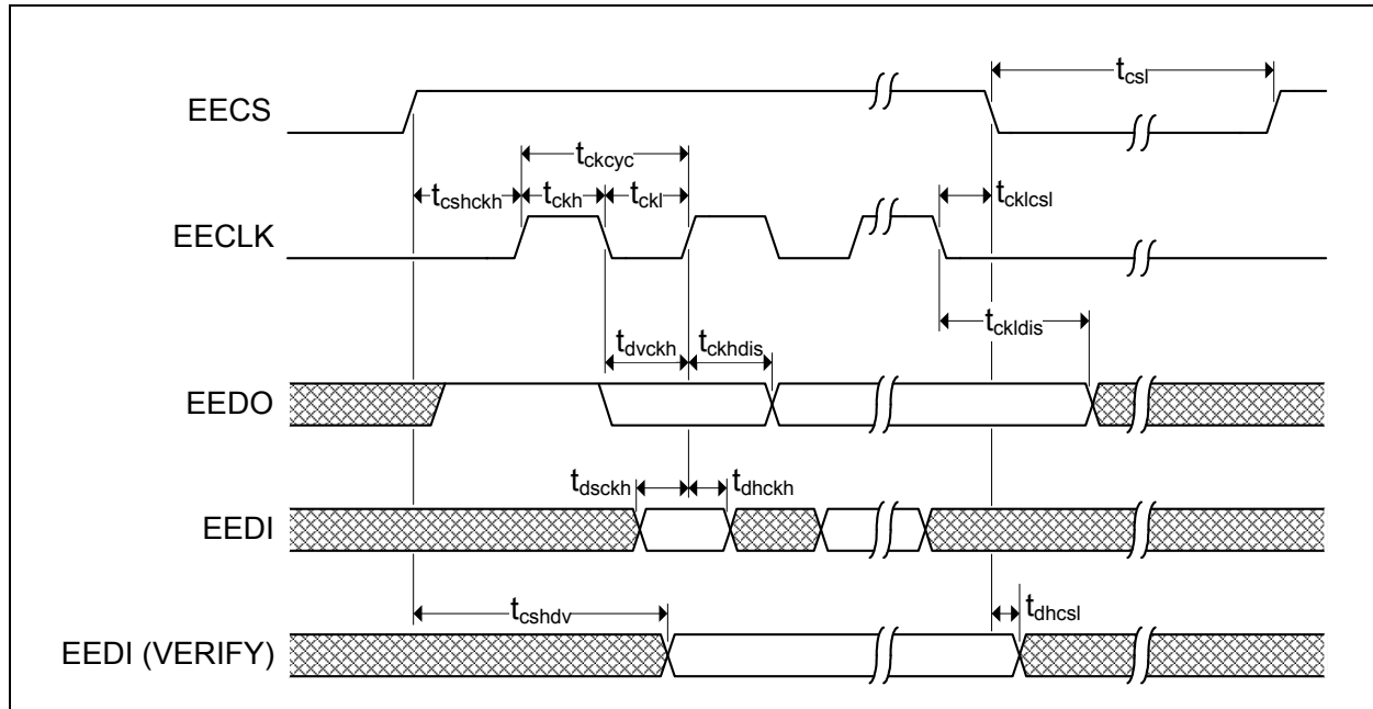
FIGURE 8-4: EEPROM TIMING
