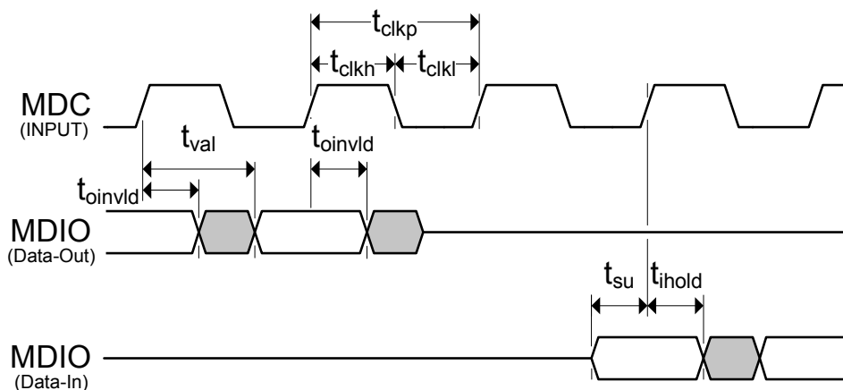
Figure 5.7 SMI Timing
