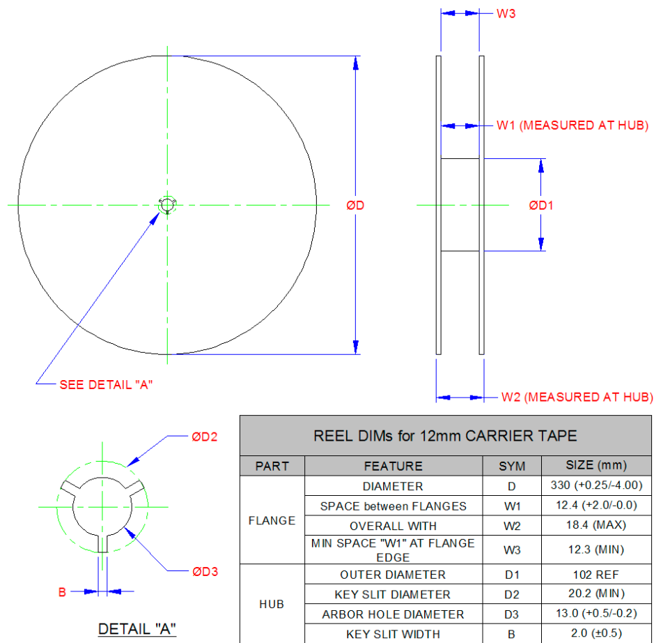
Figure 6.4 Reel Dimensions
