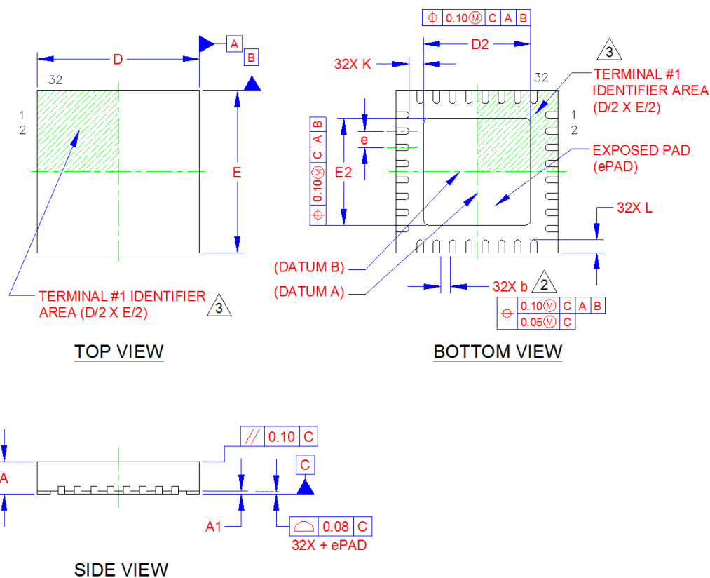
Figure 6.1 32-SQFN Package
