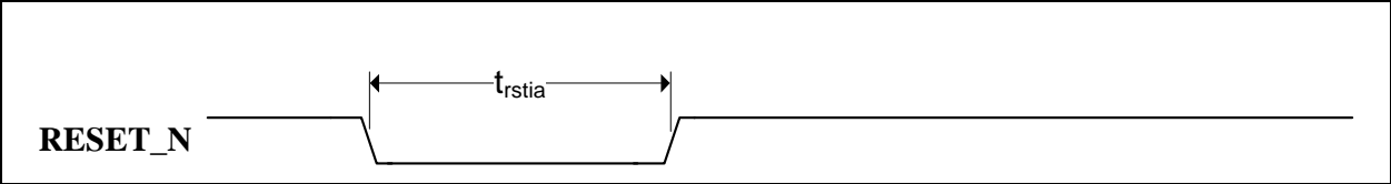
FIGURE 4-2: RESET_N TIMING
