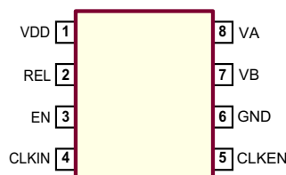
8-Lead MSOP (MG)
