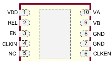
10-Lead DFN (K7)
