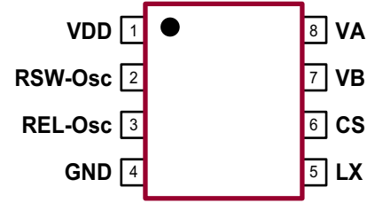
8-Lead MSOP (top view)
