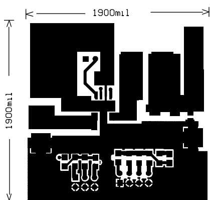
Figure 5c. Top Layer
