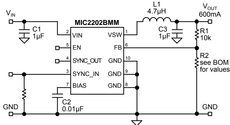
Figure 8. MIC2202BMM Schematic
