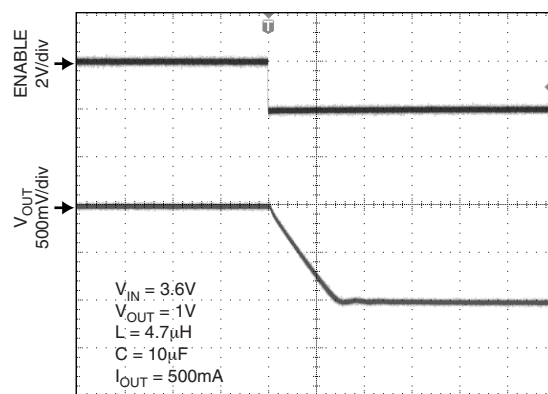
Disable Transient
