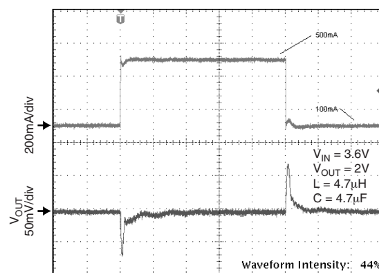
Load Transient
