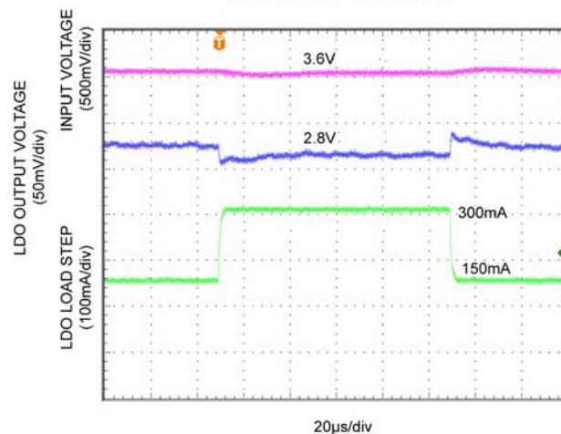
LDO Load Transient
