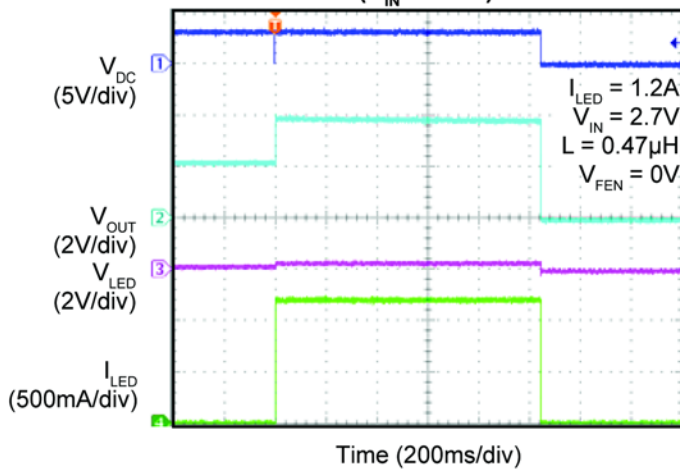
V_{OUT} Over-Voltage Protection (Over-voltage during Start-up)
