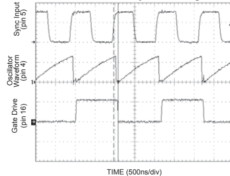
Figure 6. Sync Waveform
