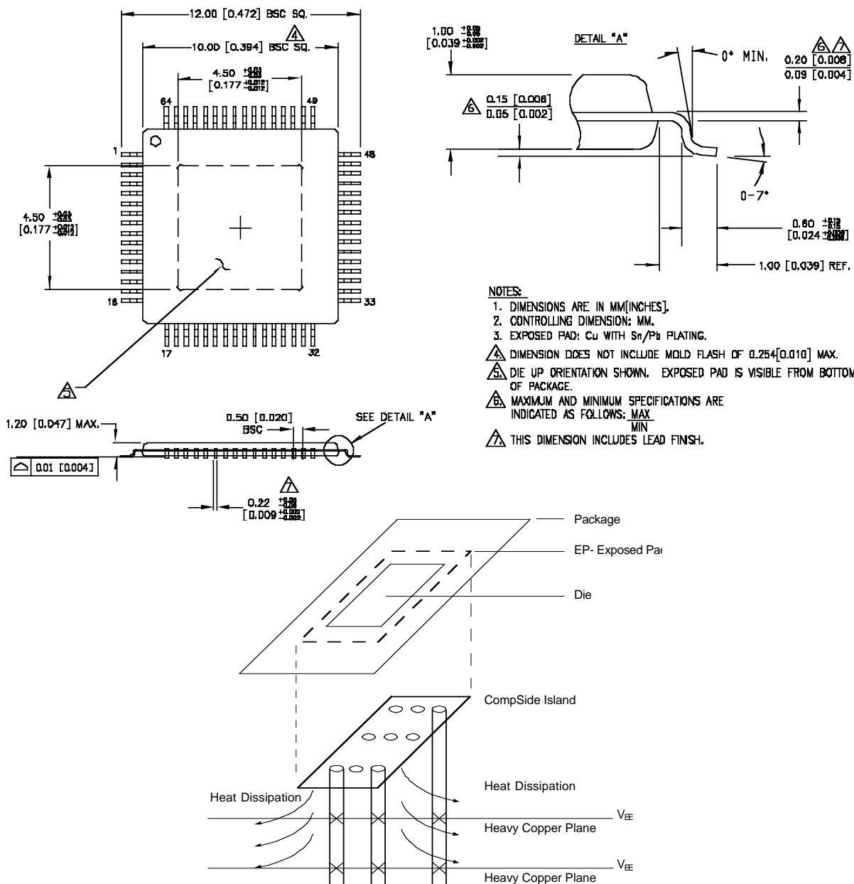
PCB Thermal Consideration for 64-Pin EPAD-TQFP Package
