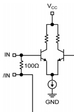
Figure 1. Simplified Differential Input Buffer
