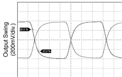
TIME (300ps/div.)
