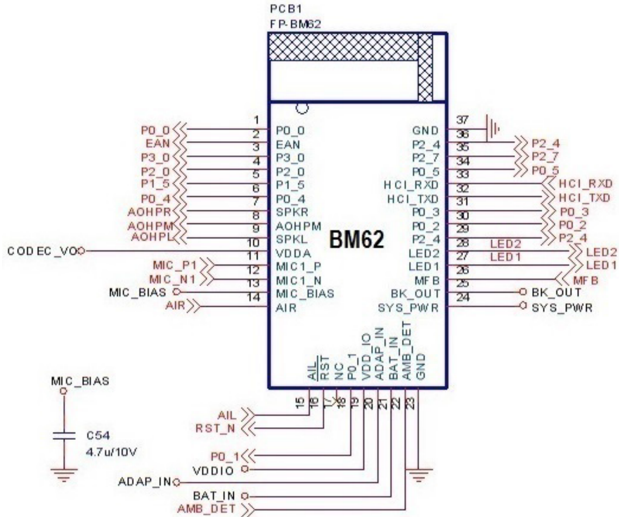
FIGURE 5-11: BM62 REFERENCE CIRCUIT FOR STEREO HEADSET APPLICATION
