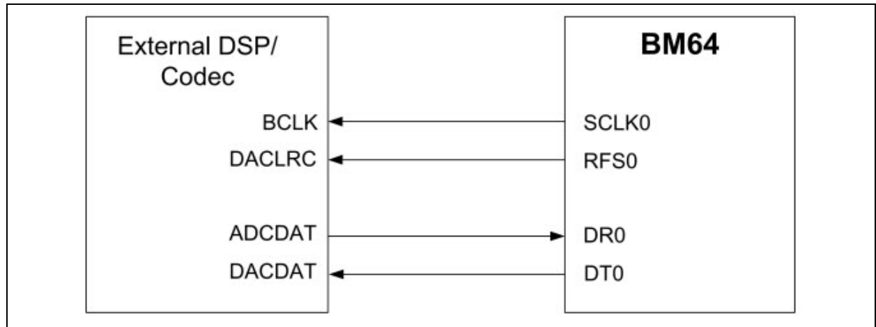
FIGURE 5-8: BM64 MODULE IN I 2 S MASTER MODE
