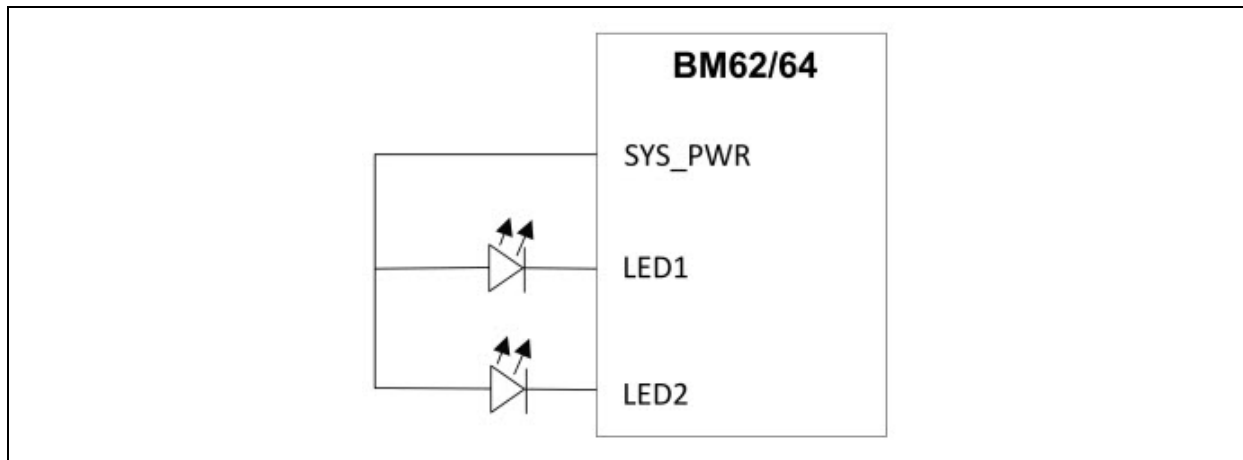
FIGURE 4-2: LED DRIVER
