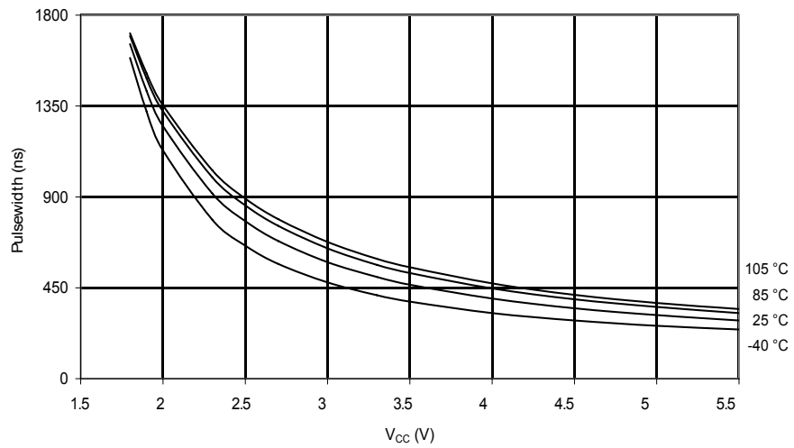
Figure 30-47. Minimum Reset Pulswidth vs. V_{CC}
