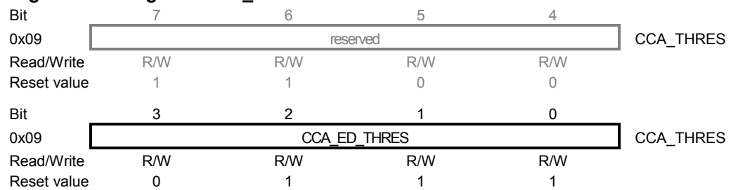
Figure 8-24. Register CCA_THRES.
