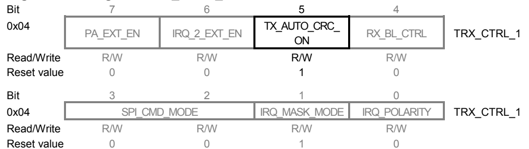
Figure 7-19. Register TRX_CTRL_1.
