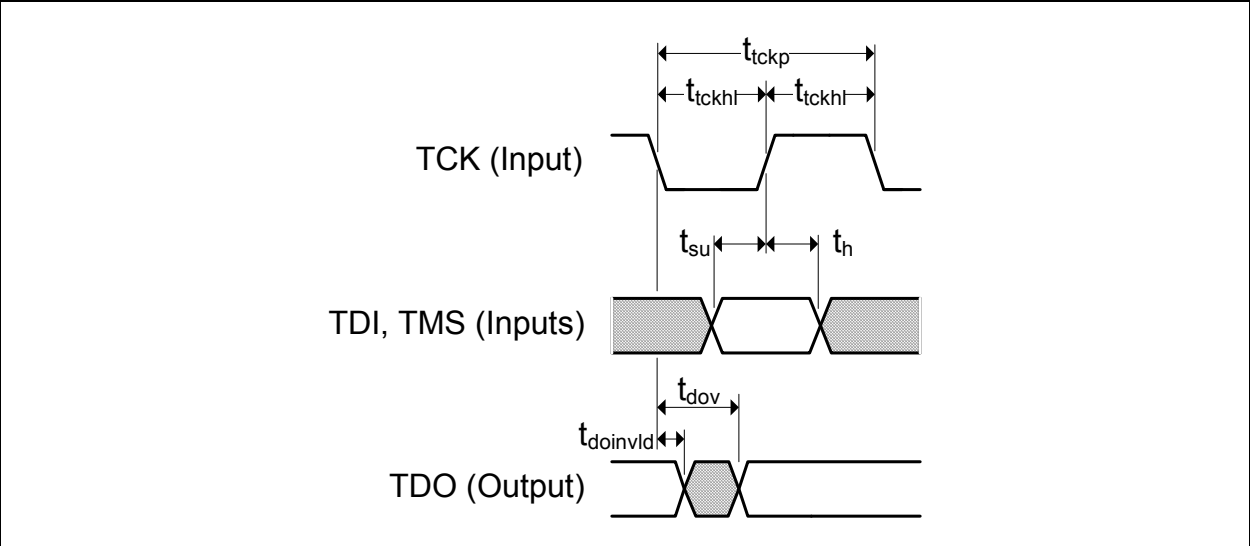
FIGURE 7-9: JTAG TIMING
