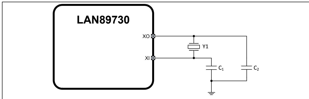
FIGURE 7-10: 300 \mu W 25 MHz CRYSTAL CIRCUIT
