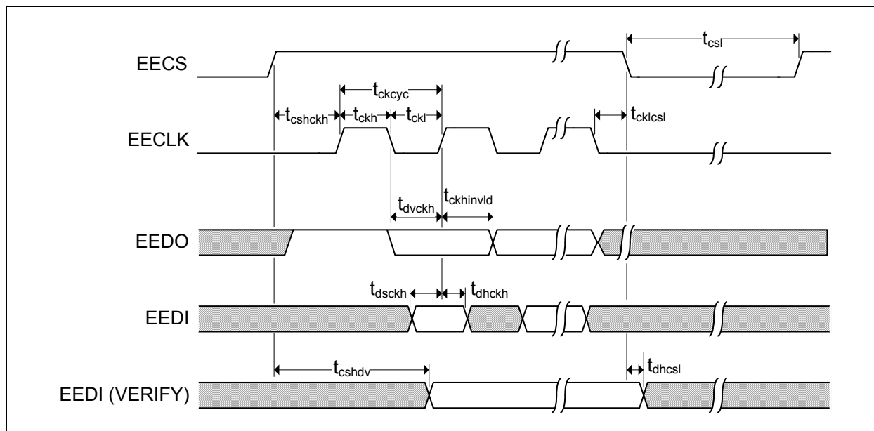
FIGURE 7-5: EEPROM TIMING
