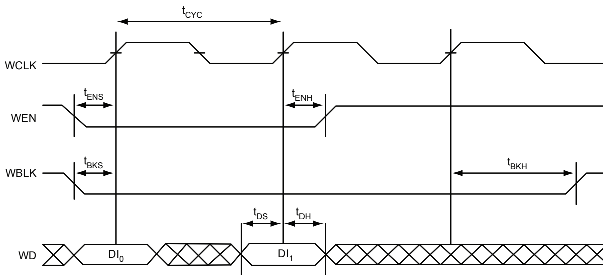
Figure 2-48 • FIFO Write
