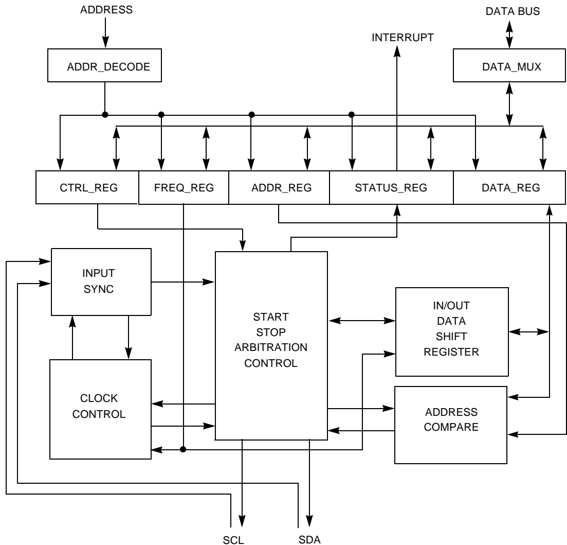
Figure 24. IIC Functional Block Diagram
