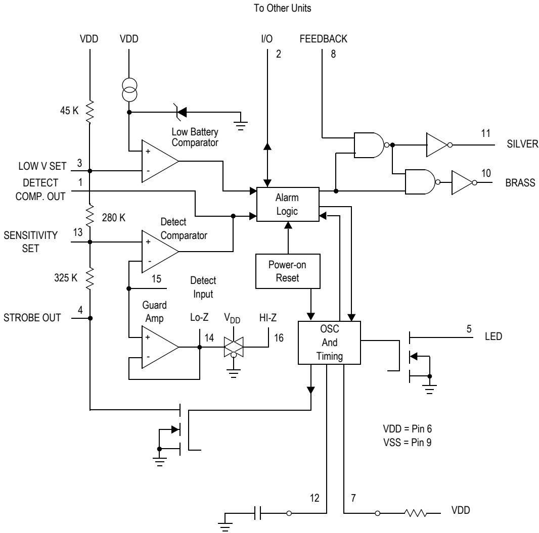
Figure 2. Block Diagram
