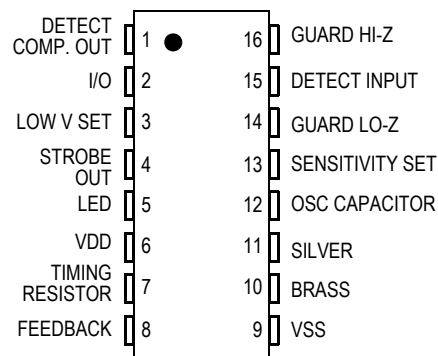
Figure 1. Pin Assignment
