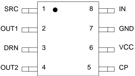
Figure 3. 33285 Pin Connections
