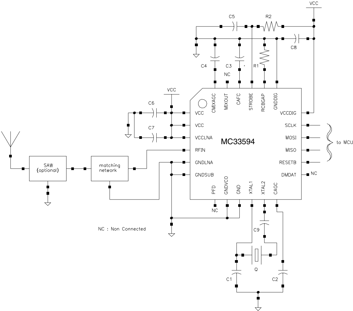
Figure 17: Application schematic
