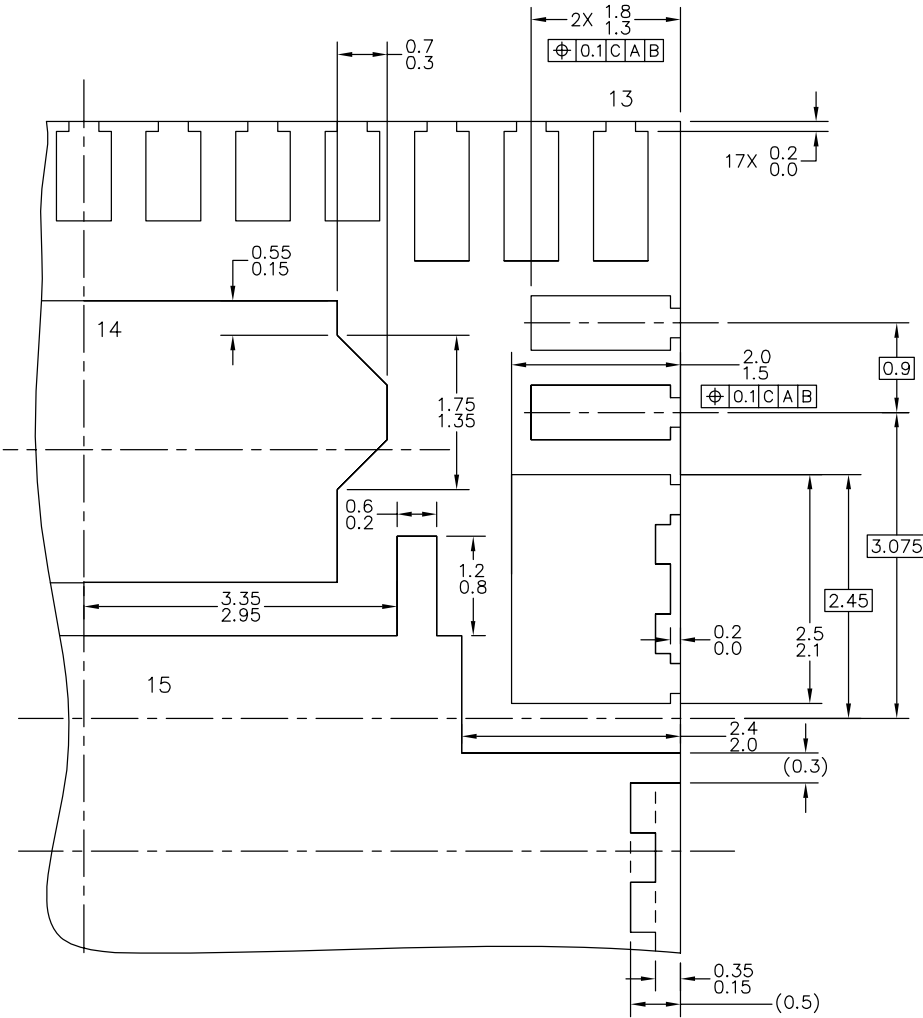
DETAIL H
