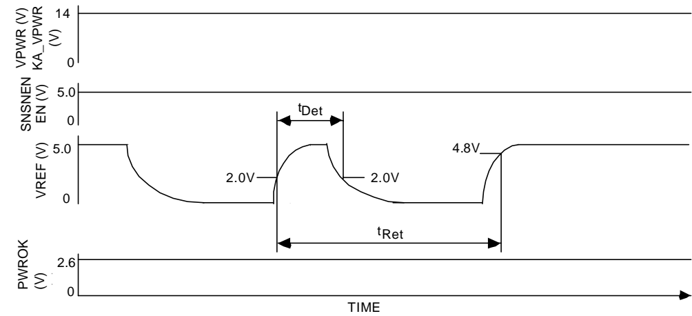
Figure 5. VREF Retry Timer
