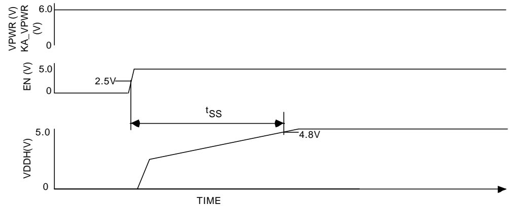
Figure 4. Soft-Start Time
