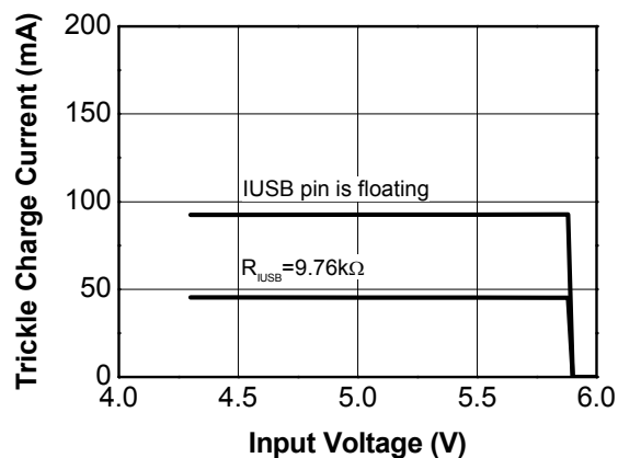
Figure 23. USB Charger Trickle Charge Current vs V_{IUSB} V_{BAT}=2.0\text{ V} , T_A=25^\circ\text{C}
