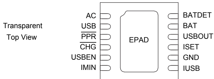
Figure 3. 34676 Pin Connections
