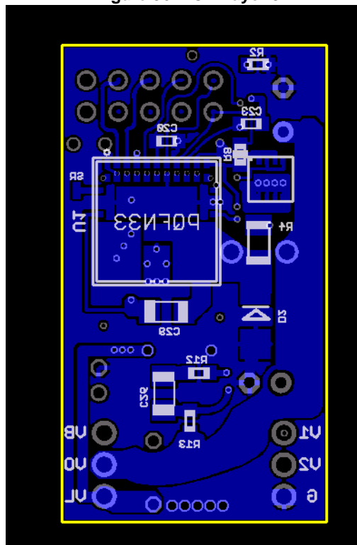
Figure 37. PCB Layer 4
