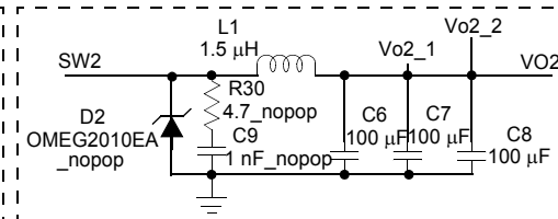
Buck Converter 2
