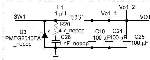
Buck Converter 1
