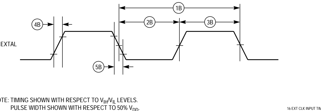
Figure A-2 External Clock Input Timing Diagram
