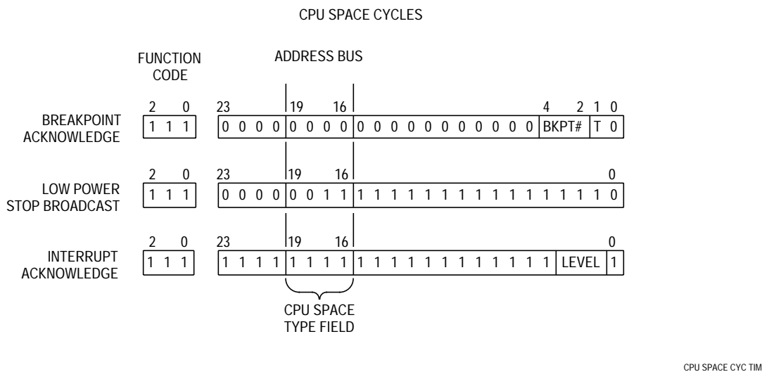
Figure 5-14 CPU Space Address Encoding
