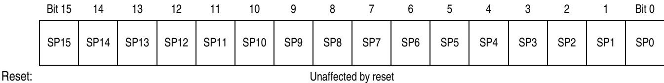
Figure 3-8. Program Counter (PC)
