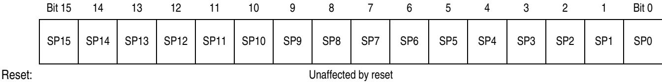
Figure 3-7. Stack Pointer (SP)
