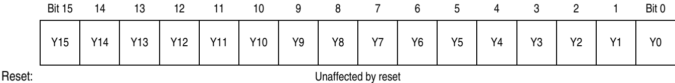
Figure 3-6. Index Register Y (Y)
