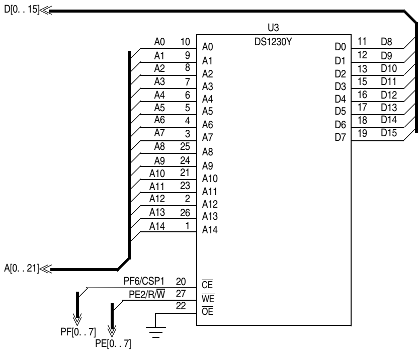
Figure 1-5. Expanded Narrow Mode SRAM Expansion Schematic (Sheet 3 of 3)
