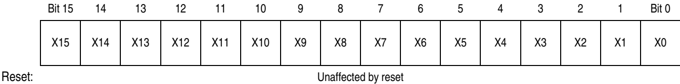
Figure 3-5. Index Register X (X)
