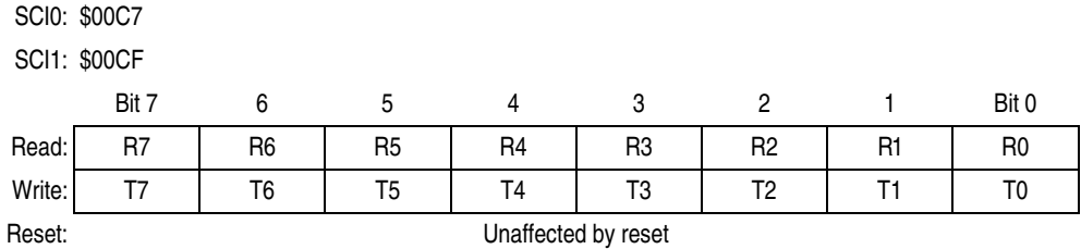
Figure 14-24. SCI Data Register Low (SC0DRL or SC1DRL)
