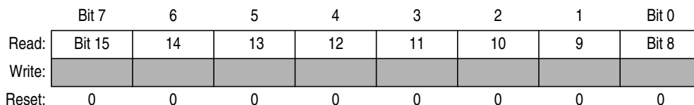
Figure 9-5. TIM Counter Registers High (TCNTH)
