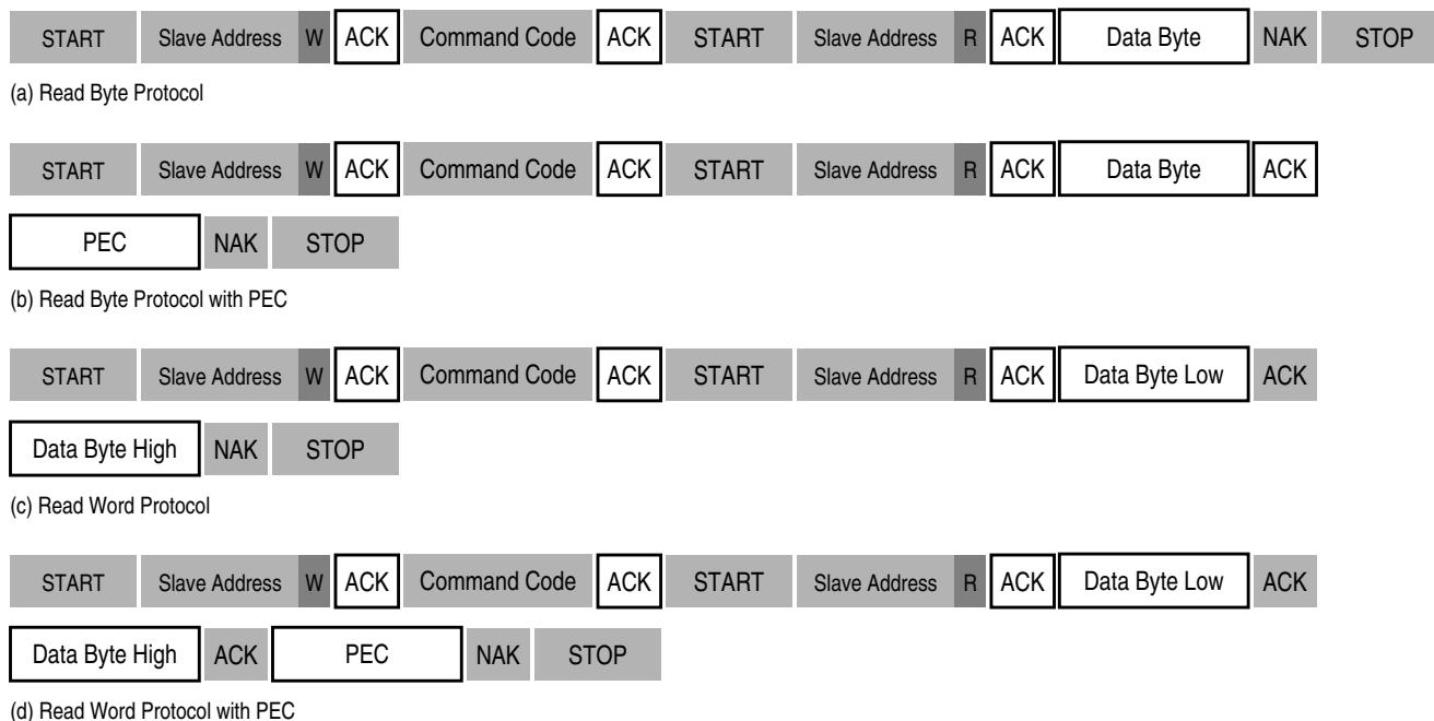
Figure 14-17. Read Byte/Word
