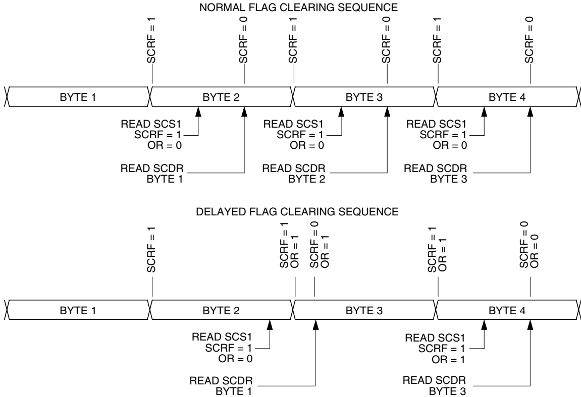
Figure 11-13. Flag Clearing Sequence
