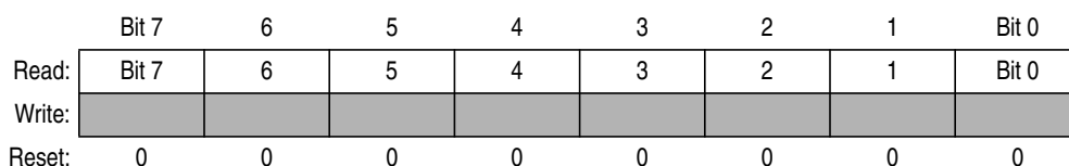
Figure 9-6. TIM Counter Registers Low (TCNTL)
