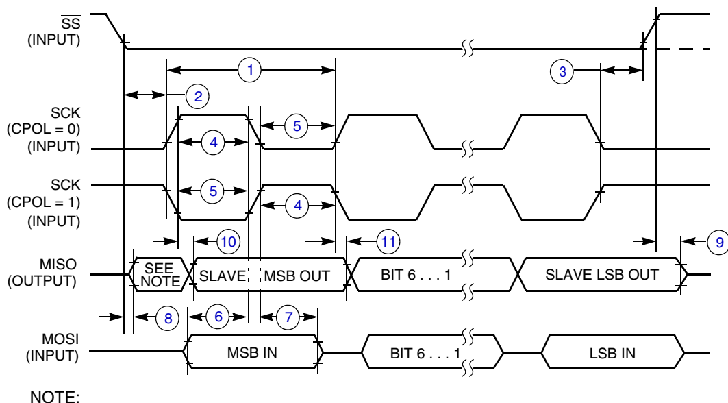
Figure A-18. SPI Slave Timing (CPHA = 1)
