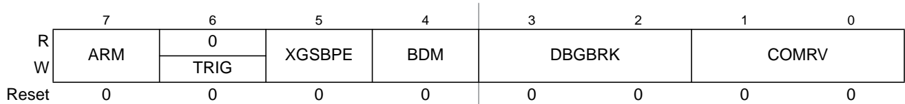
Figure 22-3. Debug Control Register (DBGC1)
